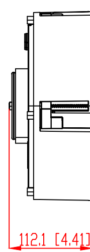
MOUNTING DEPTH
